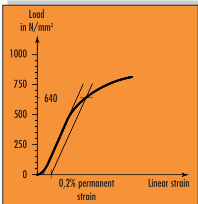
BUMAX 88: 800/640 N/mm 2
