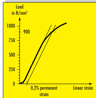
BUMAX 109: 1000/900 N/mm 2
